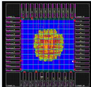
PQ-TLS ASIC Layout — TSMC 28nm, Cadence
